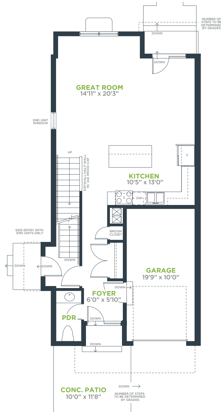
MAIN FLOOR 773 SQ.FT.
