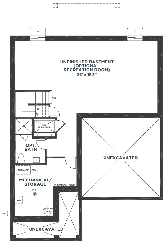
BASEMENT LEVEL
