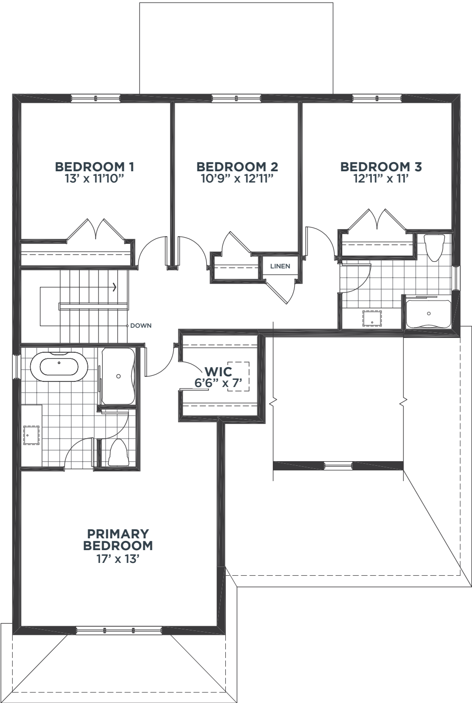
UPPER FLOOR
