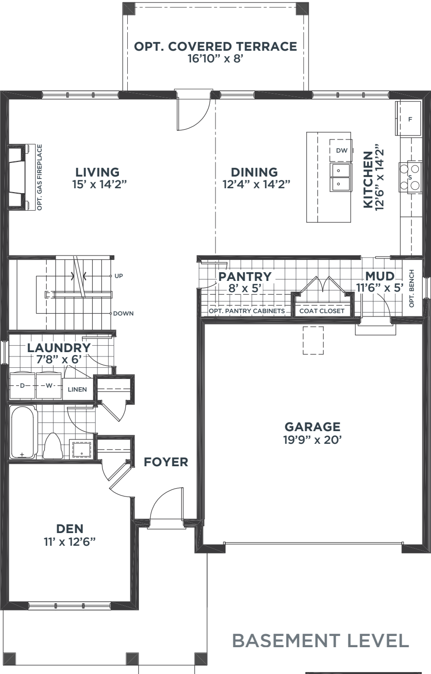
MAIN FLOOR
