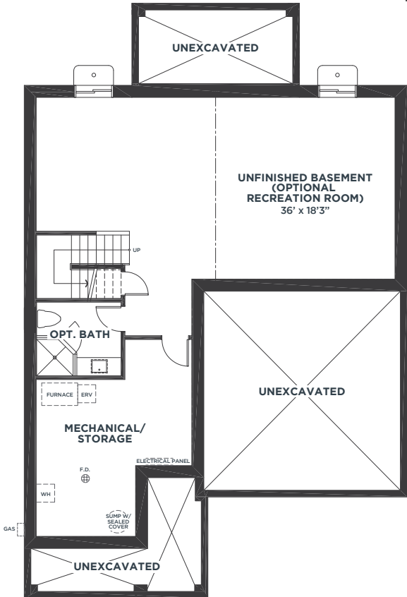
BASEMENT LEVEL
