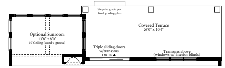
MAIN FLOOR w/ OPTIONAL SUNROOM 2105 SQ. FT.
