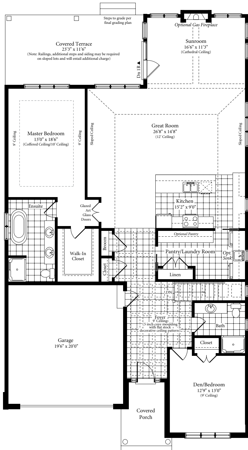
MAIN FLOOR 2080 SQ. FT.
