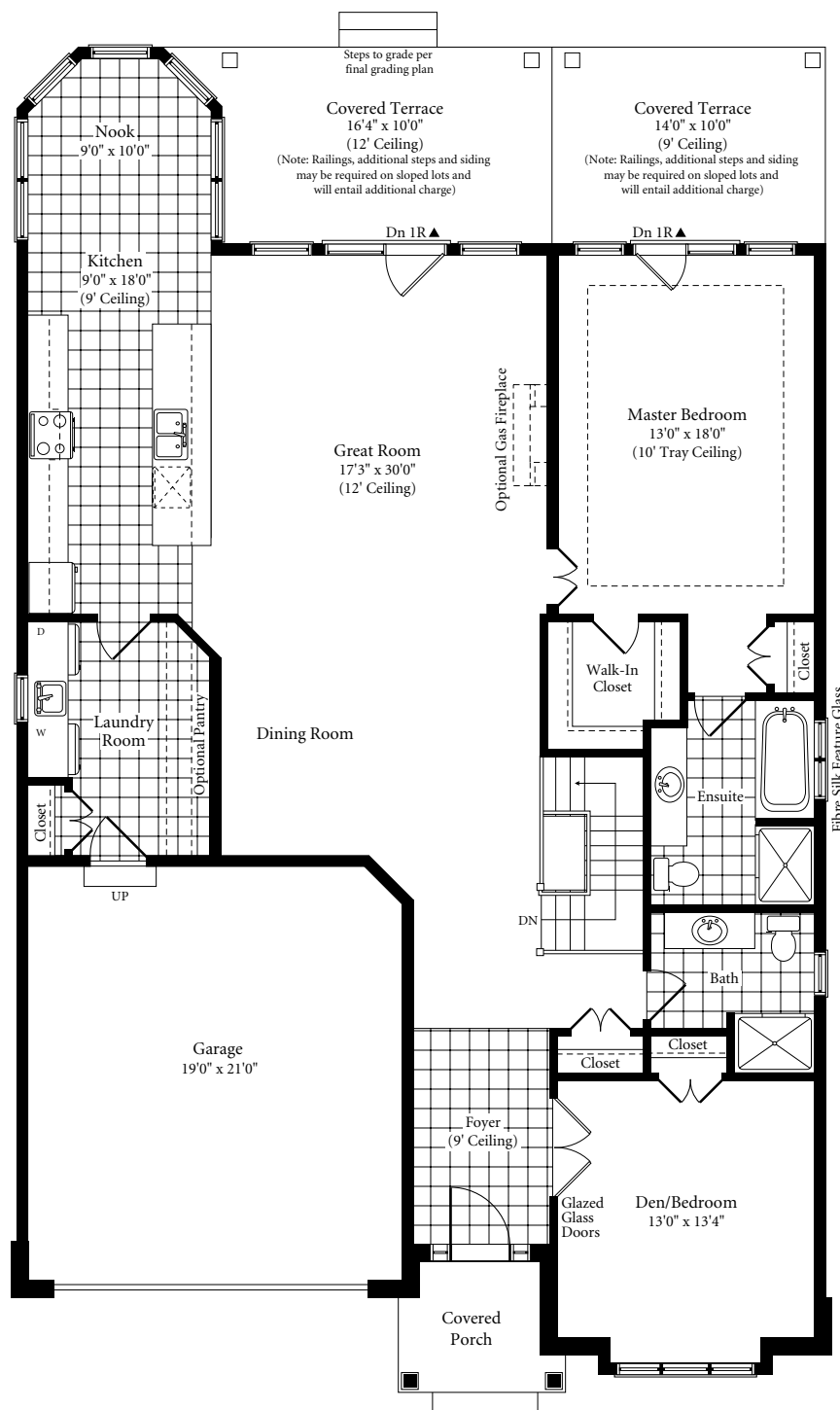
MAIN FLOOR 1870 SQ. FT.
