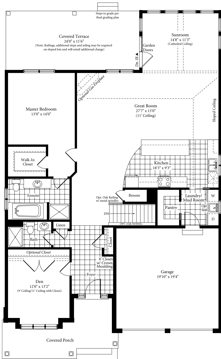
MAIN FLOOR 1833 SQ. FT.
