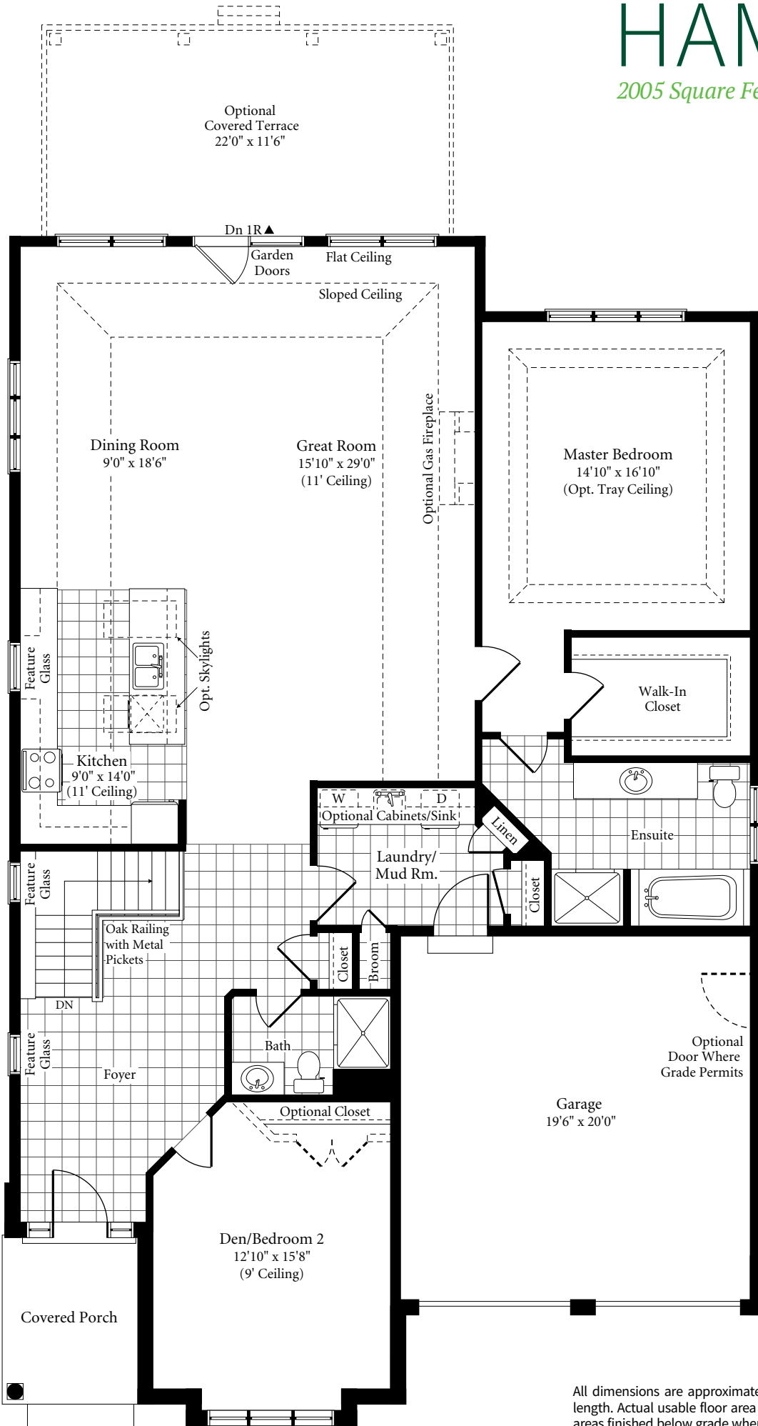
MAIN FLOOR 2005 SQ. FT.
