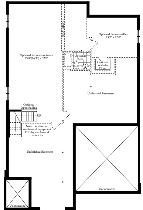
OPTIONAL FINISHED BASEMENT 1030 SQ. FT.
